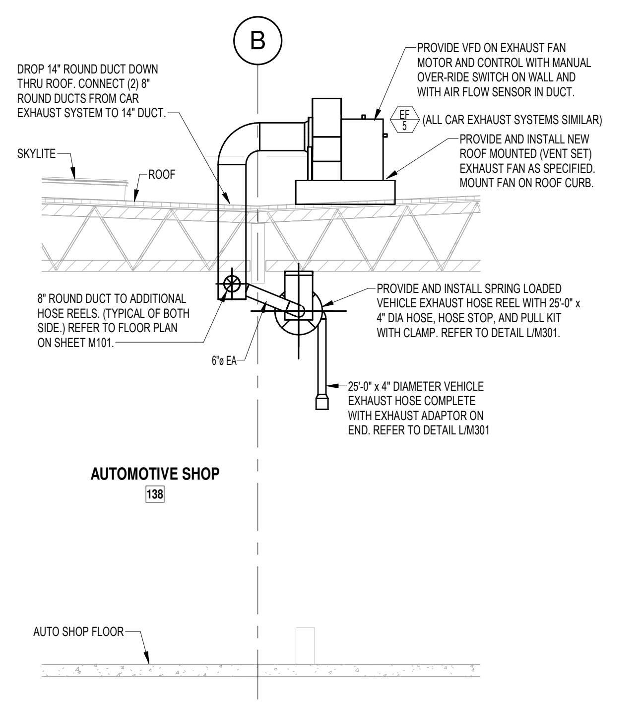
1 MECHANICAL SECTION 1 M201 1/4" = 1'-0"
