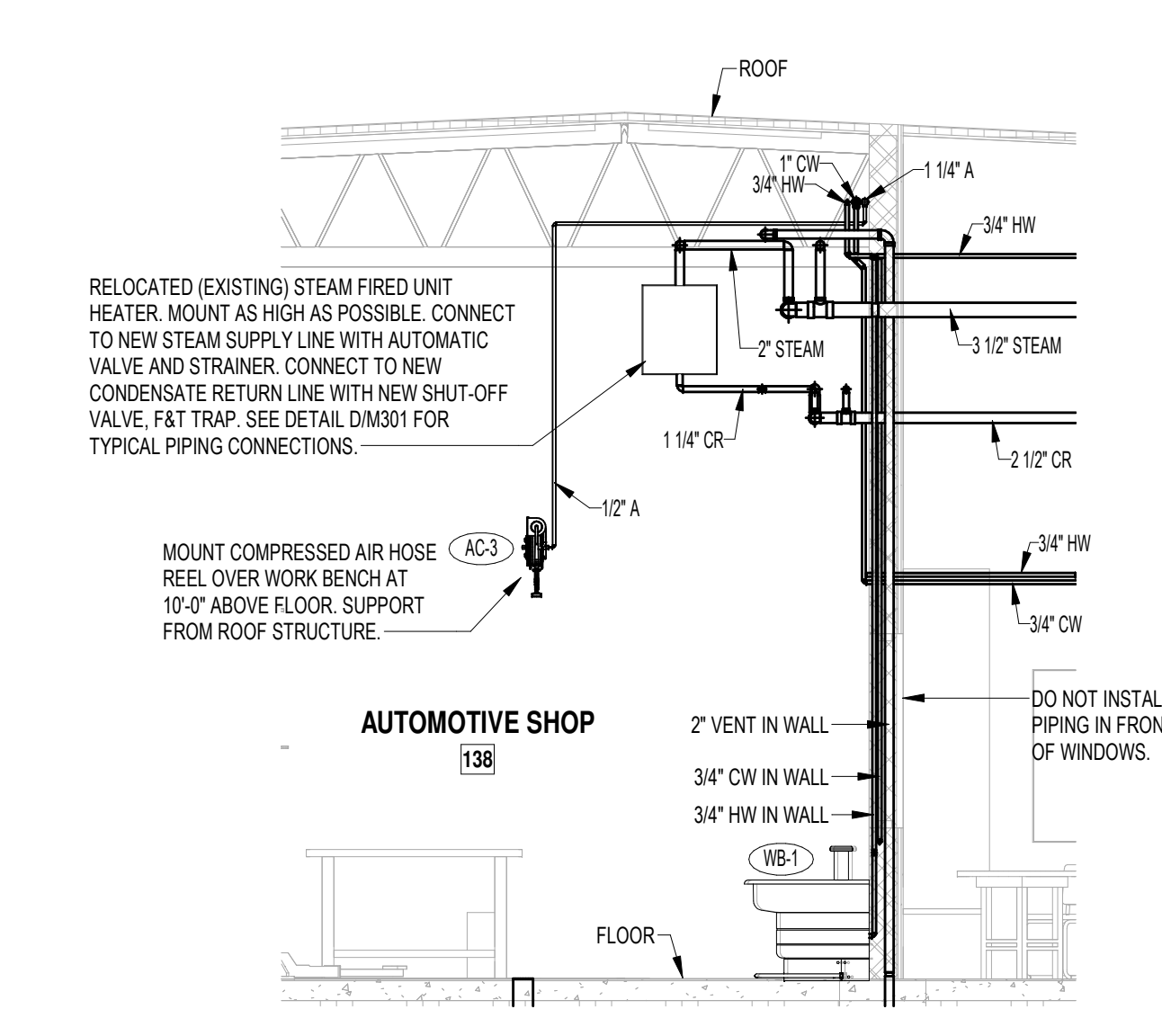
4 MECHANICAL SECTION 4 M201 1/4" = 1'-0"
