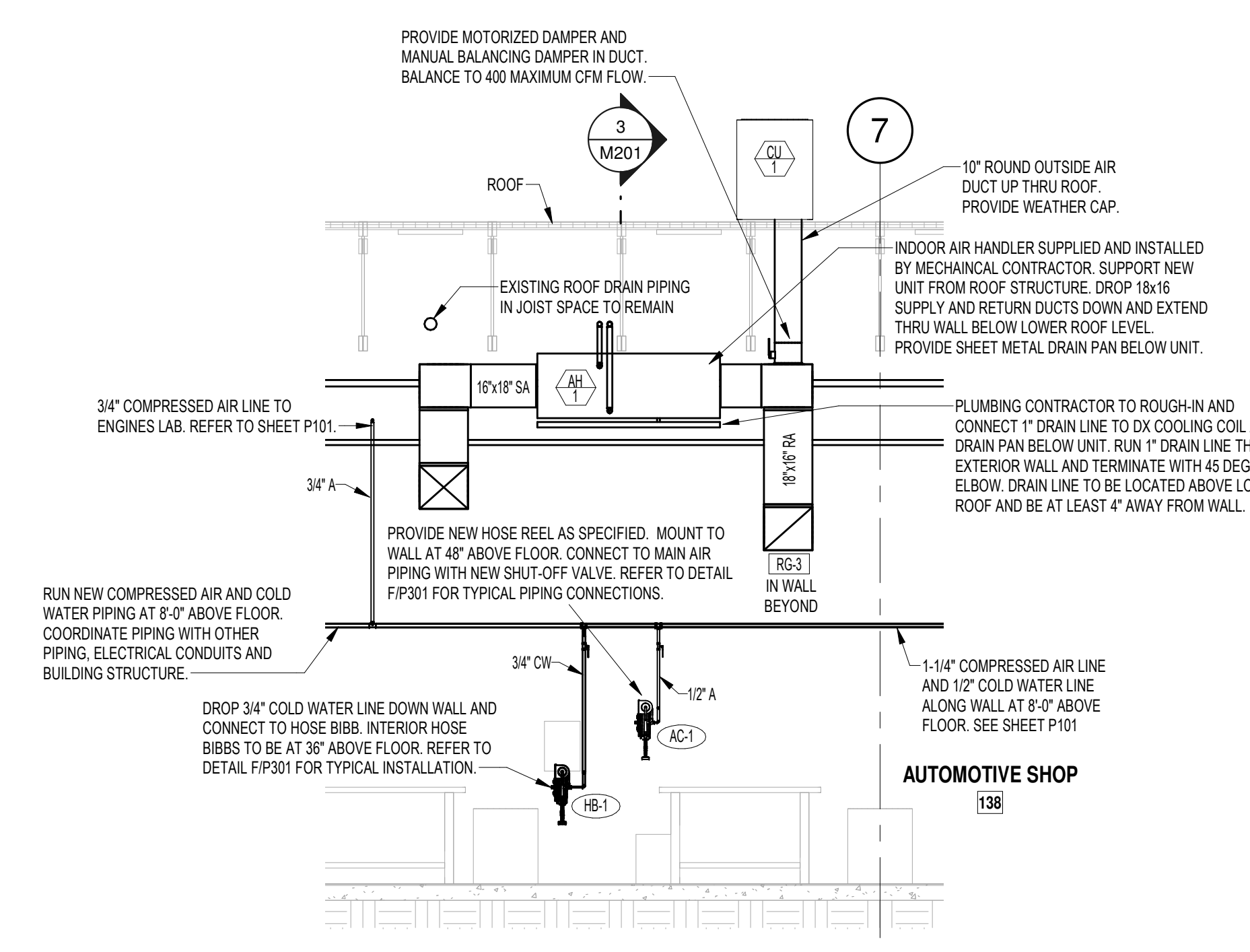
2 MECHANICAL SECTION 2 M201 1/4" = 1'-0"
