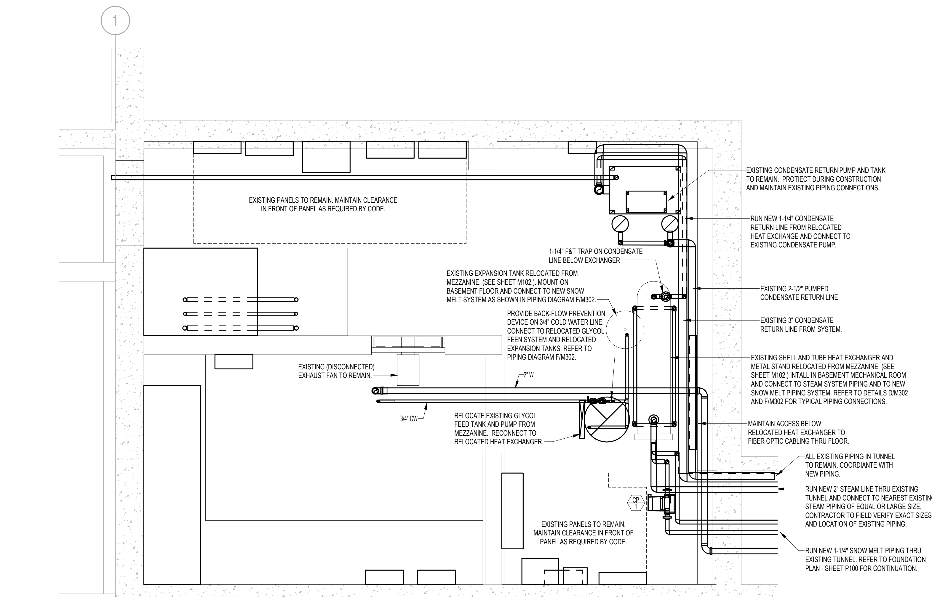
5 BASEMENT MECHANICAL ROOM M201 1/2" = 1'-0"
