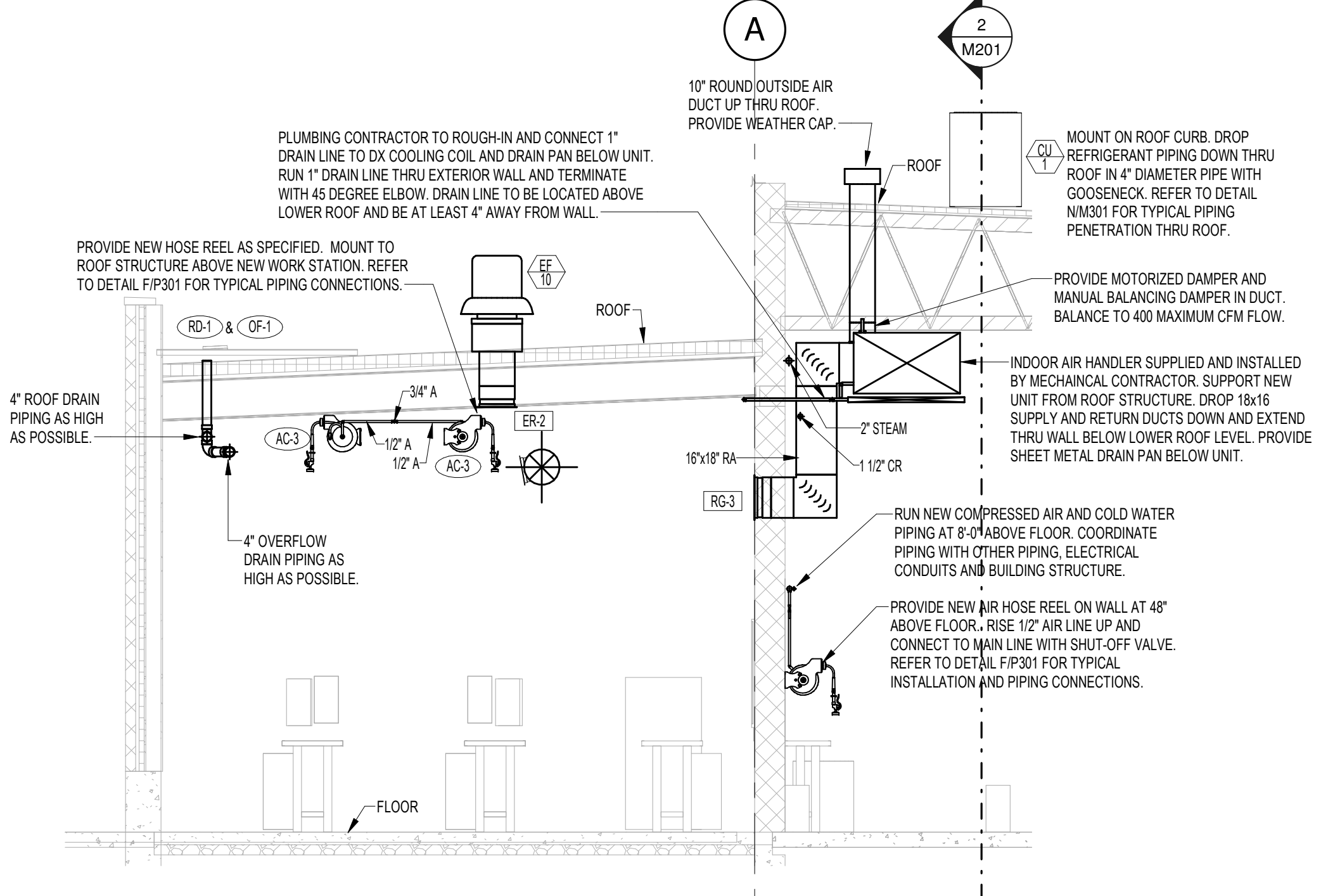
3 MECHANICAL SECTION 3 M201 1/4" = 1'-0"
