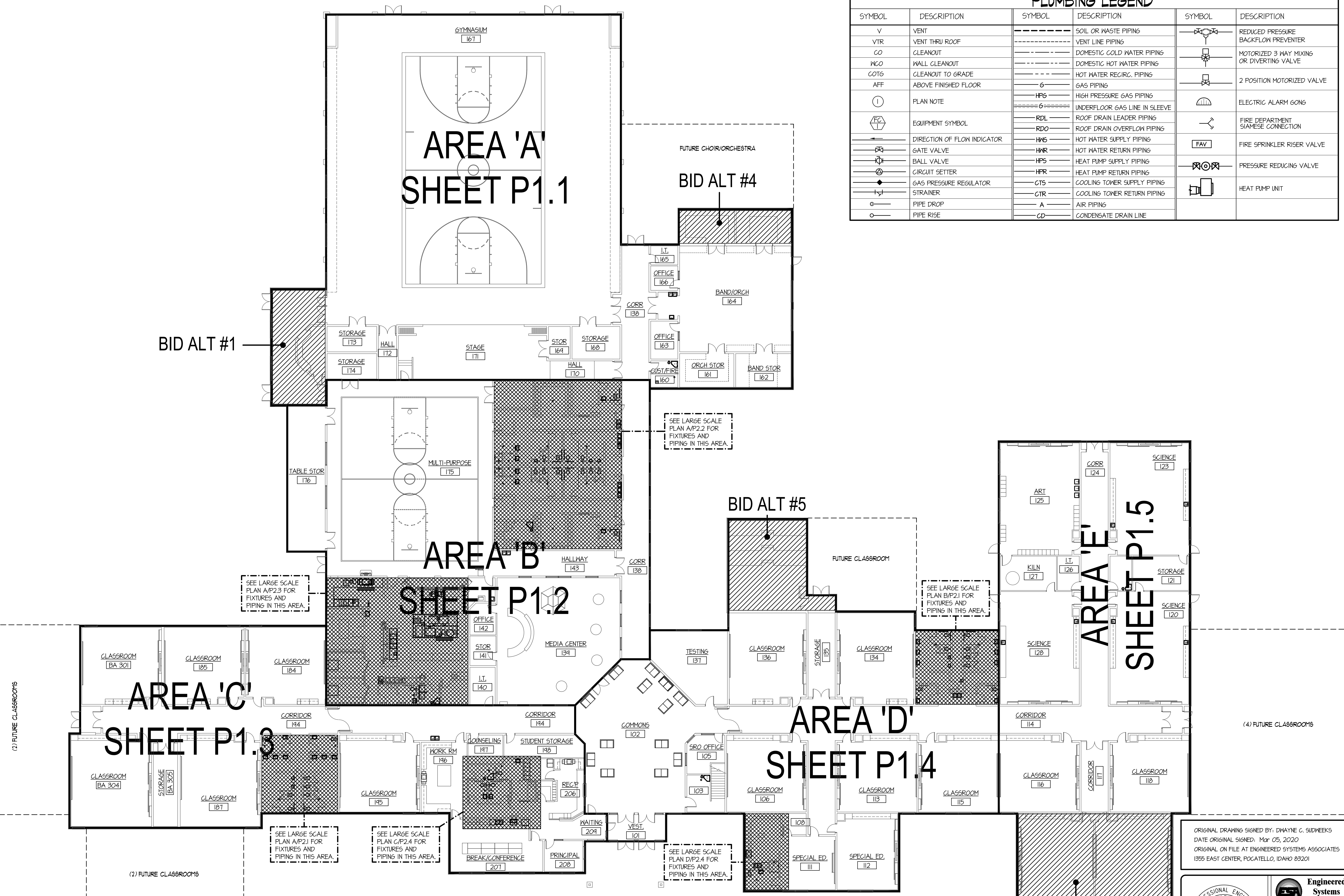
COMPOSITE PLUMBING FLOOR PLAN SCALE: 1/16" = 1'-0"
