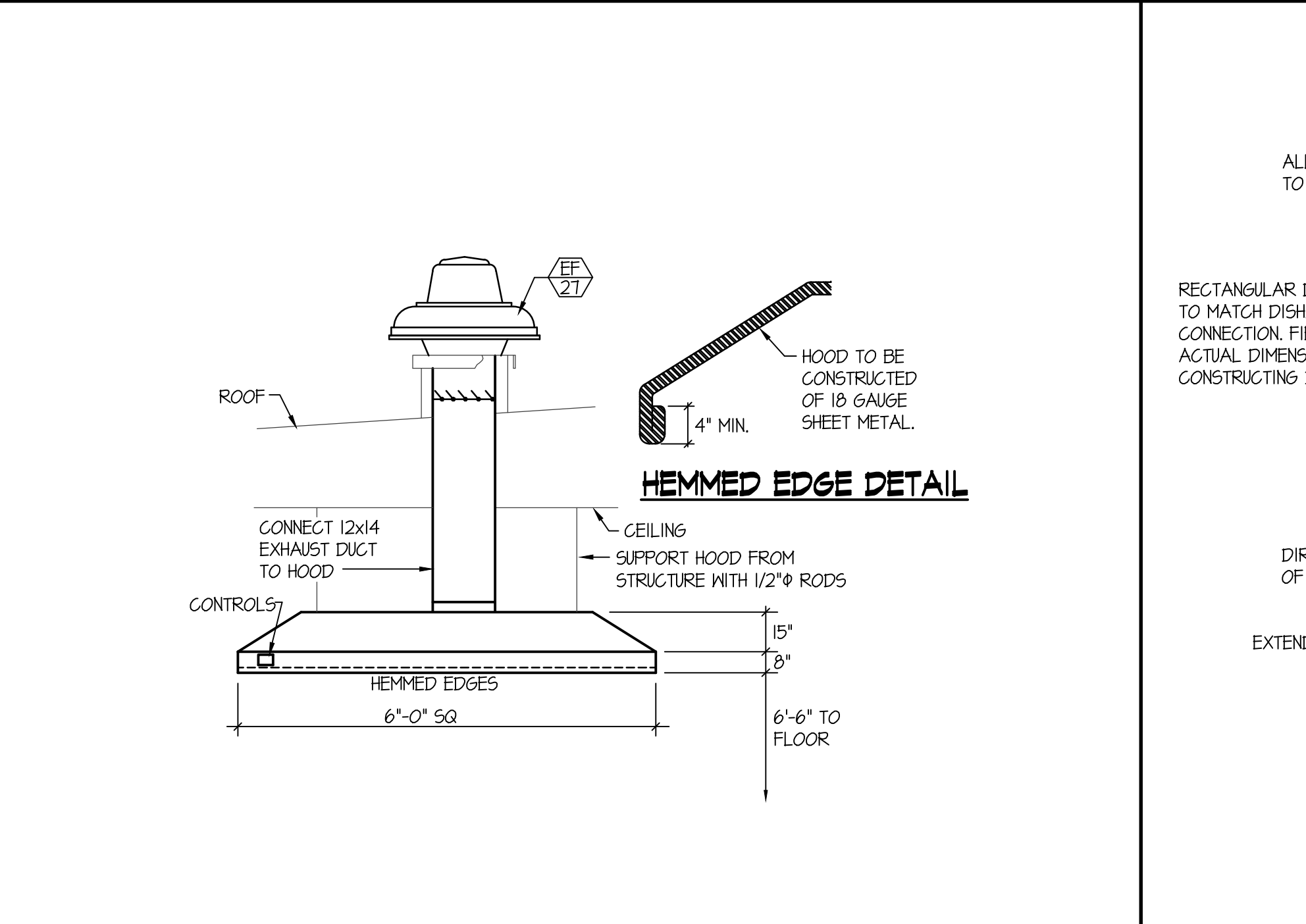
M CANOPY HOOD DETAIL NO SCALE
