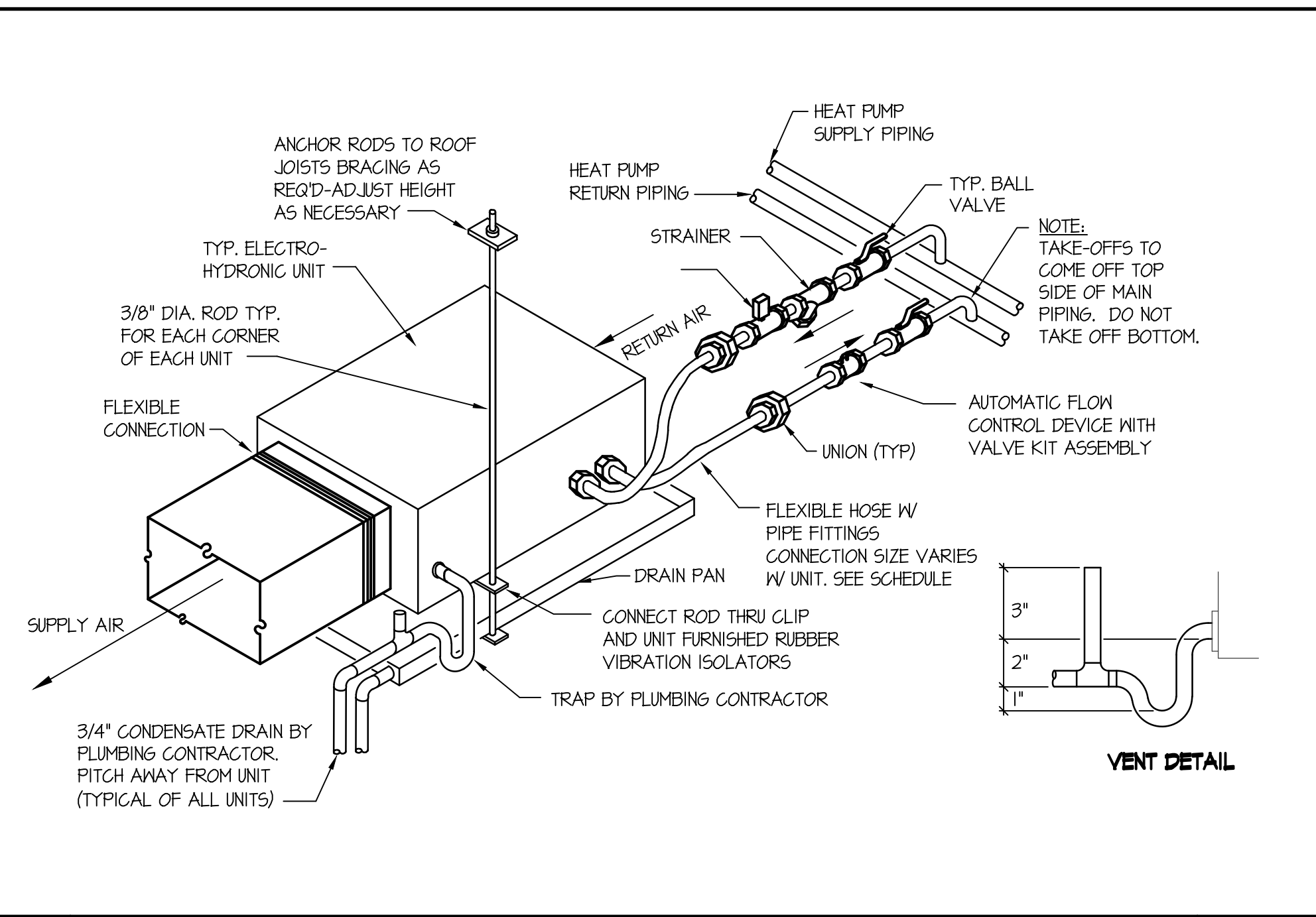
A HEAT PUMP PIPING WITH AUTOMATIC 2-WAY VALVE NO SCALE
