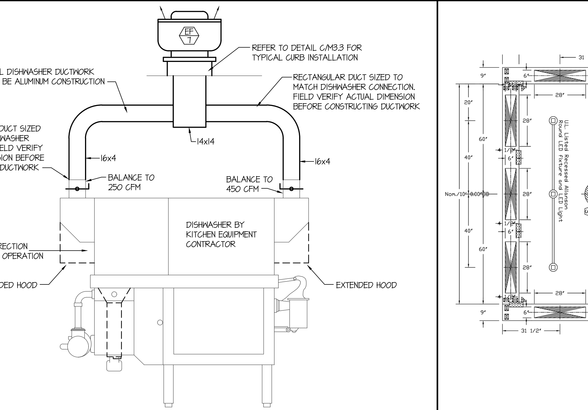
N DISHWASHER HOOD DETAIL NO SCALE
