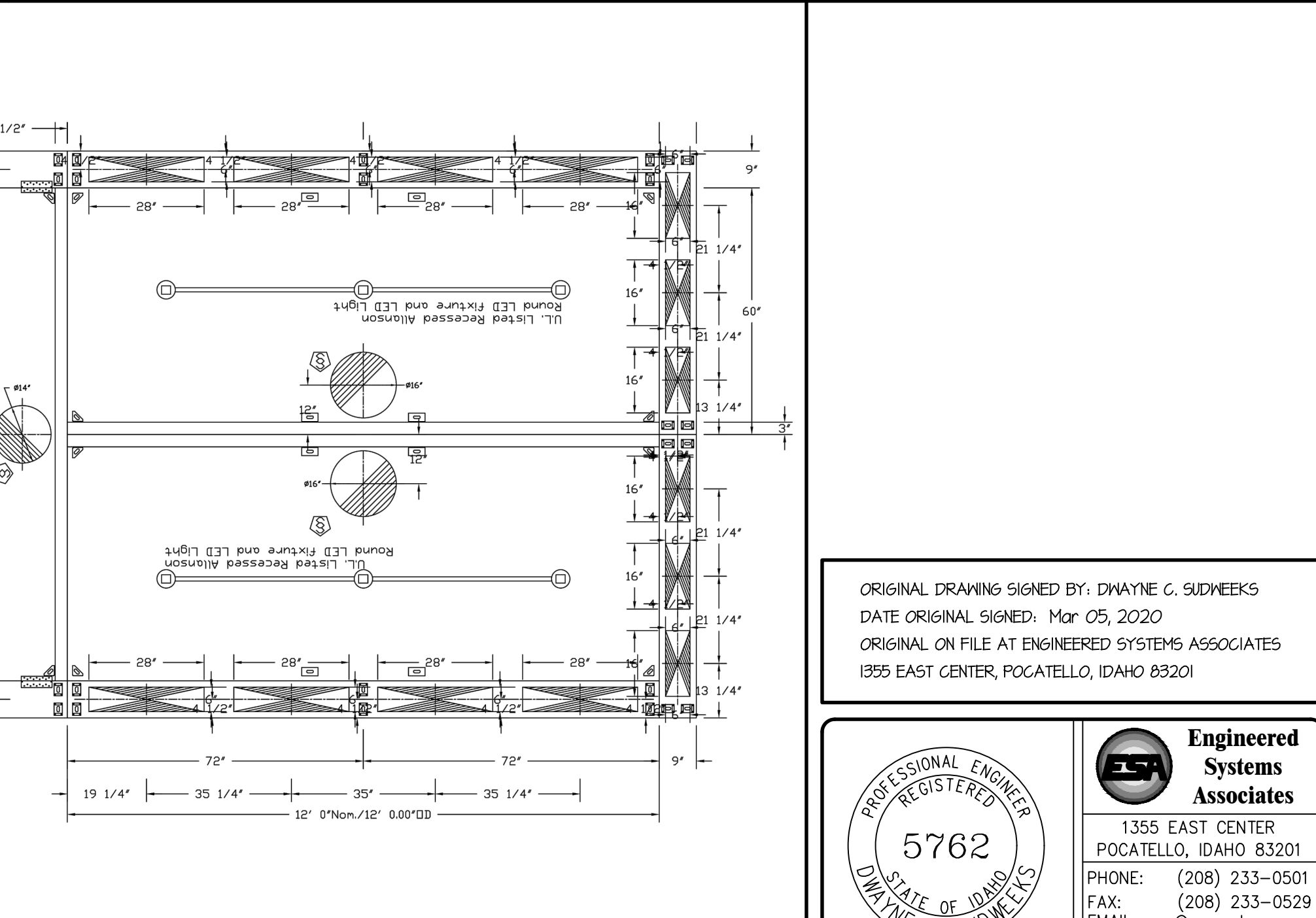
O KITCHEN HOOD DUCT CONNECTION DETAIL NO SCALE
