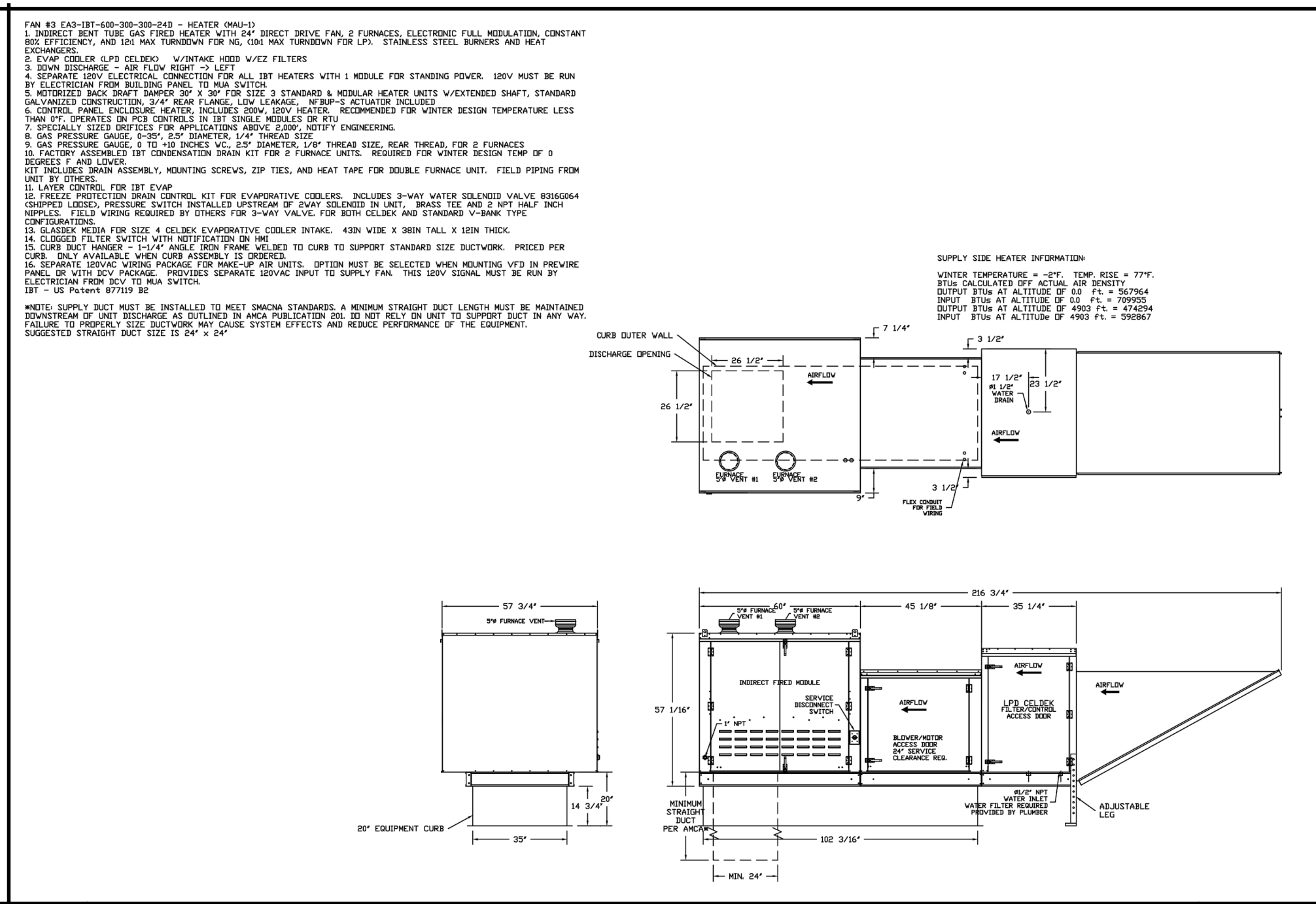
C KITCHEN HOOD MAKE-UP AIR UNIT DETAIL NO SCALE
