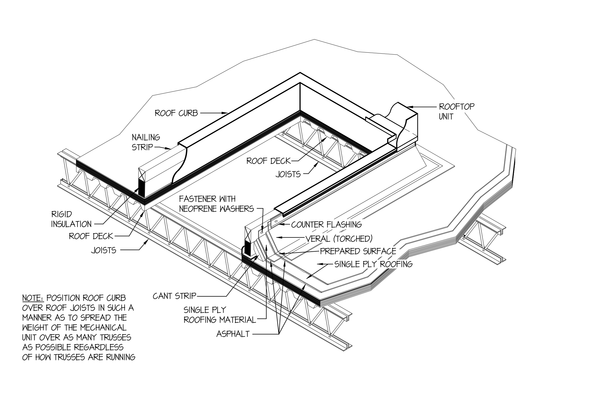
D TYPICAL ROOF EQUIPMENT MOUNTING DETAIL NO SCALE
