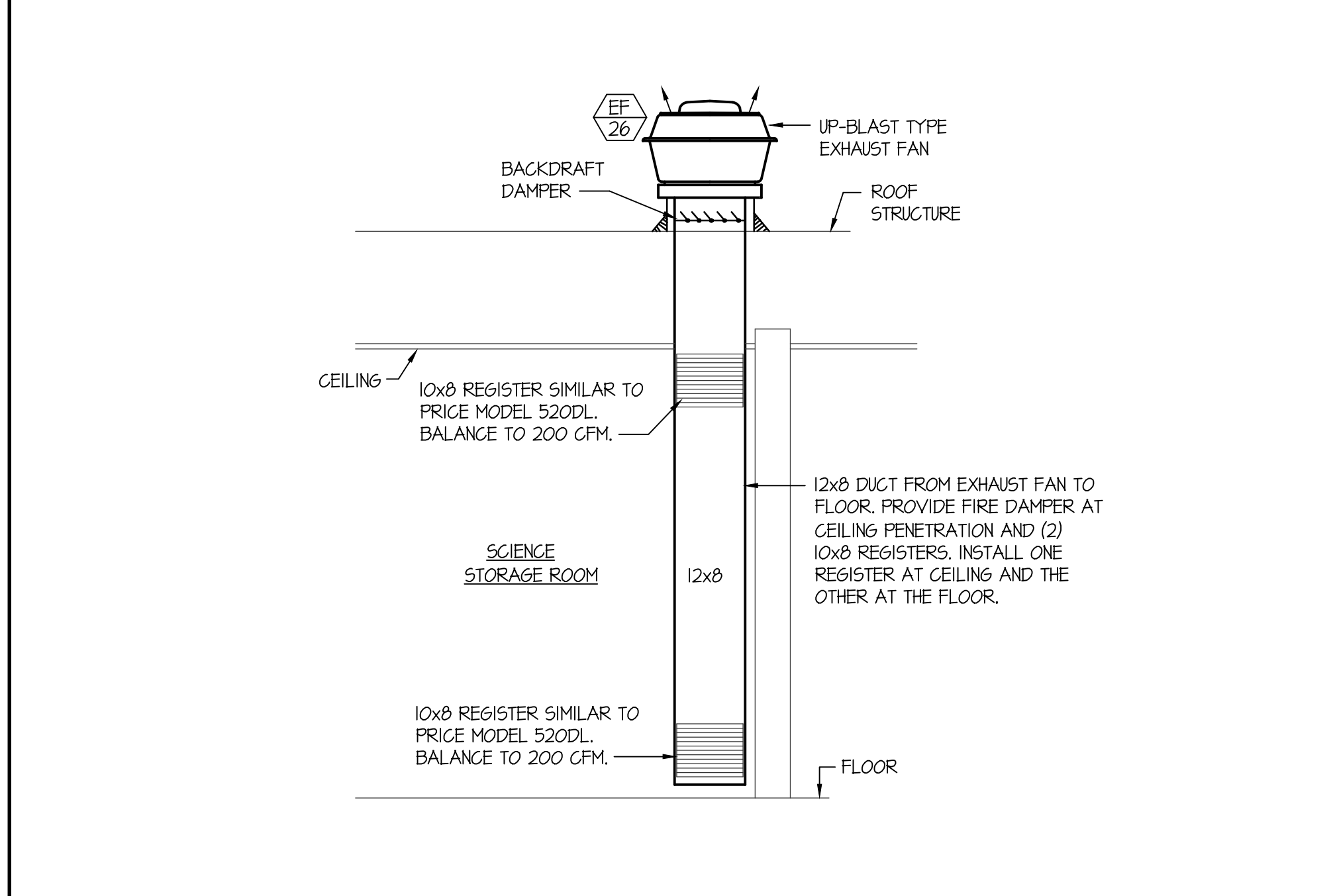
E CHEMICAL STORAGE ROOM VENTILATION DETAIL NO SCALE
