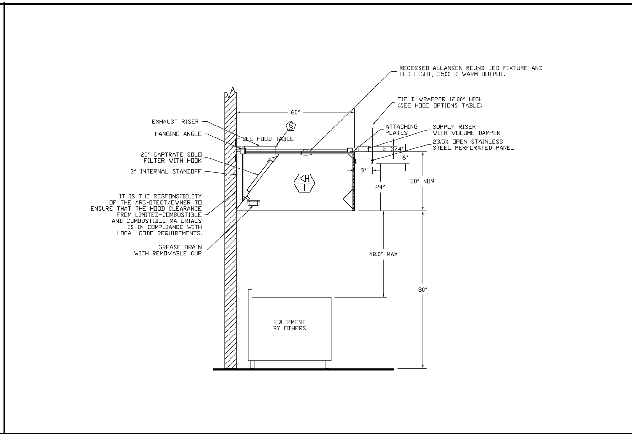
B TYPICAL KITCHEN HOOD SECTION NO SCALE
