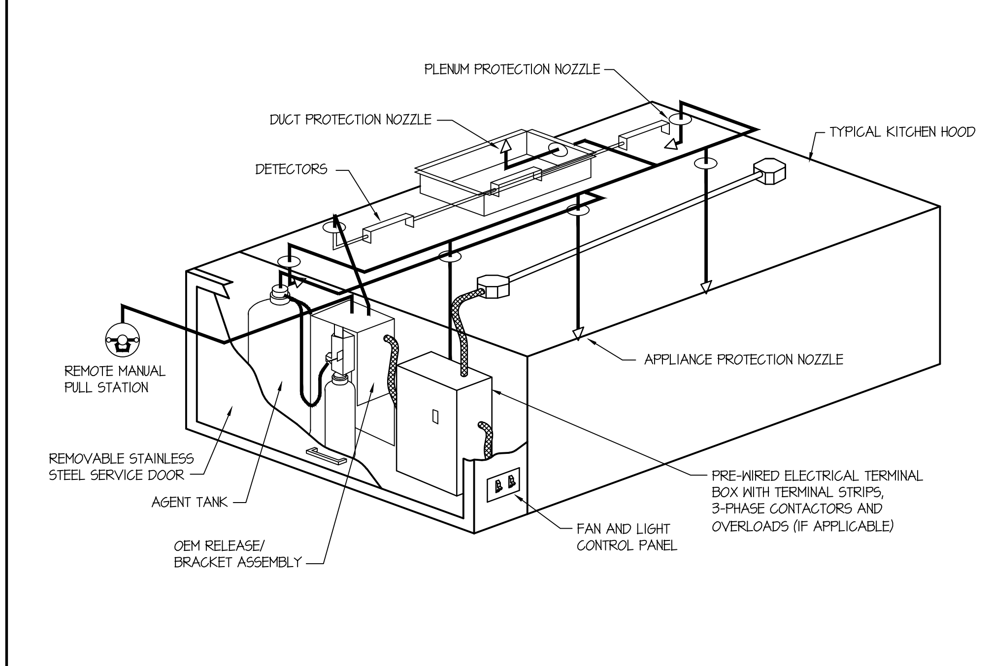
F TYPICAL ANSUL R-102 SYSTEM LAYOUT NO SCALE
